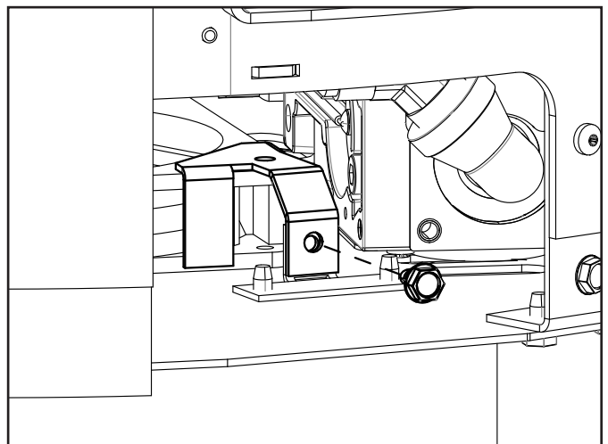
Figure 26: Fan Retainer Detachment
