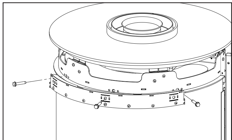
Figure 20: Glass Top/Bottom Retainer
