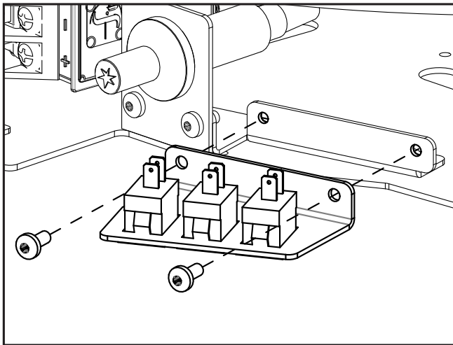
Figure 88: Rocker Switch Mount Disconnect from Firebox
