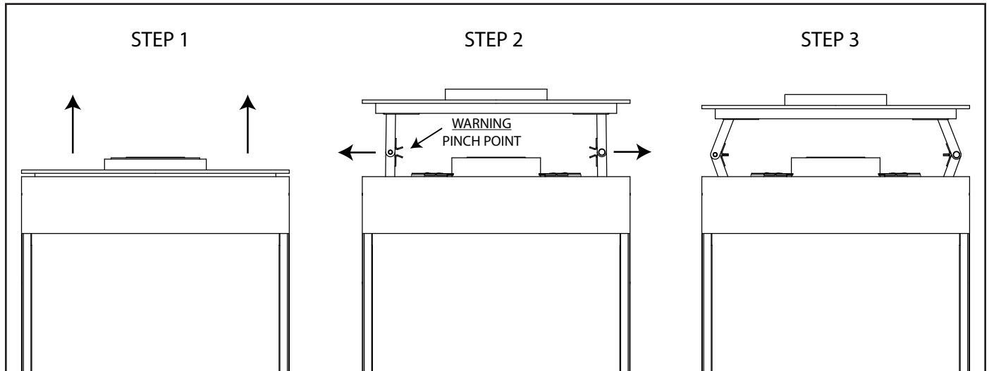
Figure 10: Lifting the Top Plate
