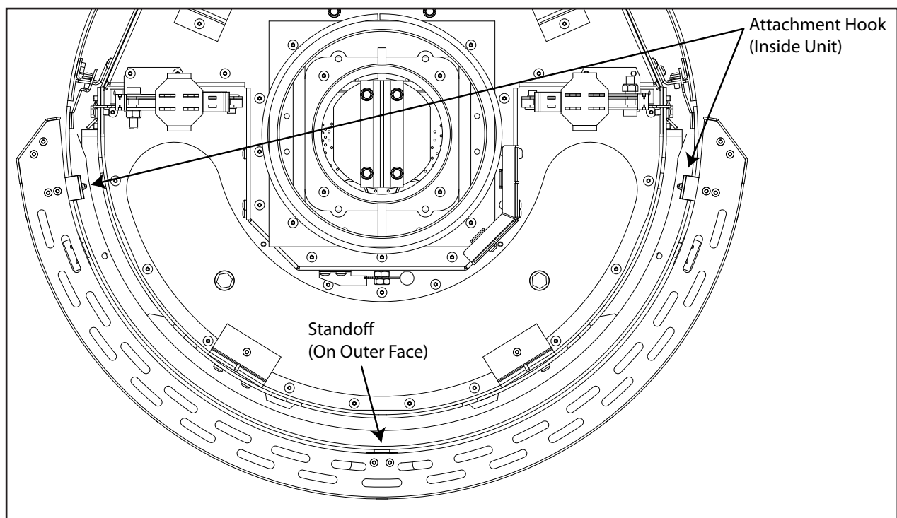
Figure 14: Safety Screen Attachment (Top-Down View)
