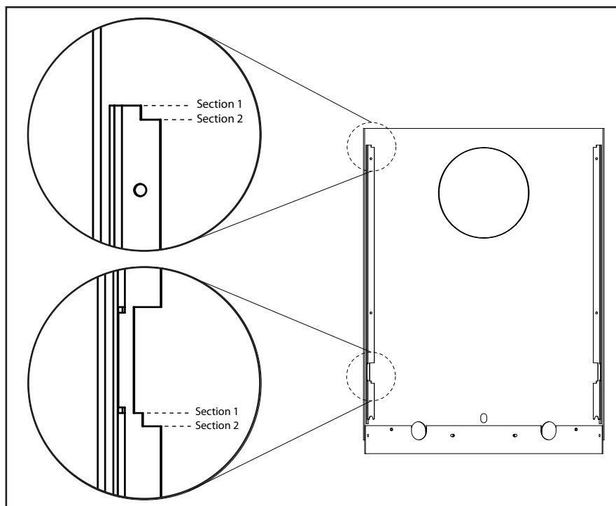
Figure 16: Chassis Mounting Slots
