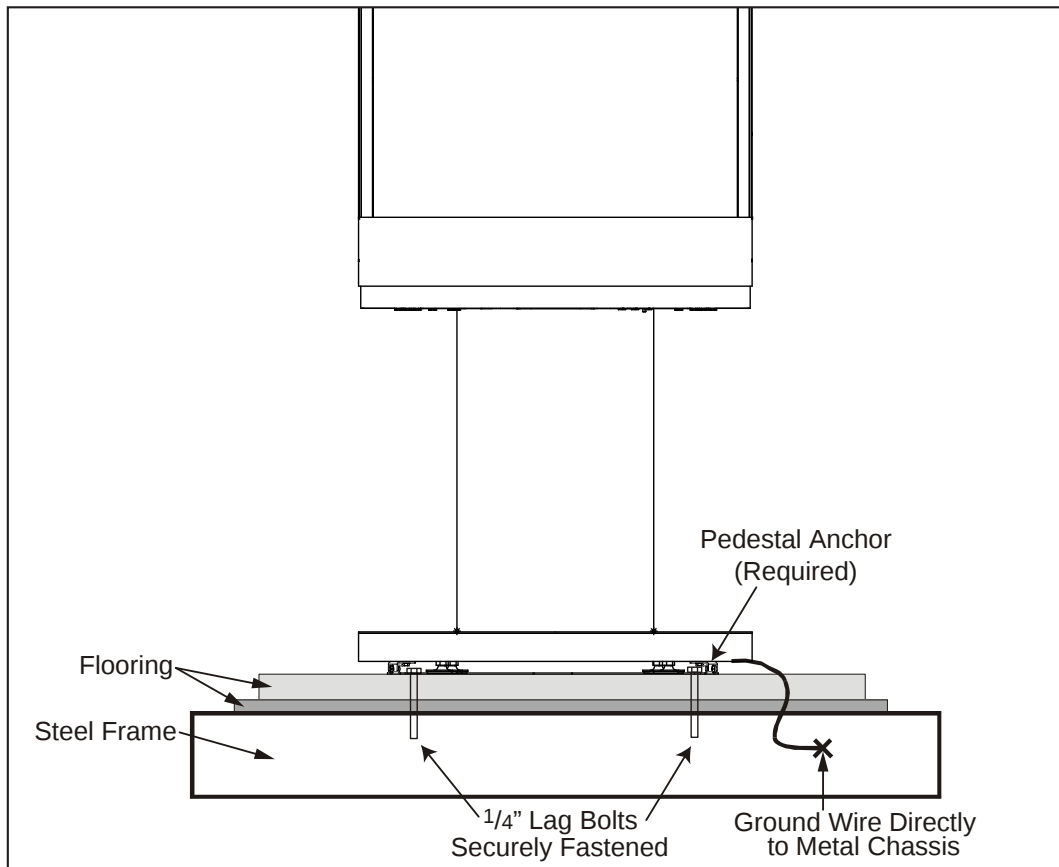
Figure 91: Correct Mobile Home Installation
