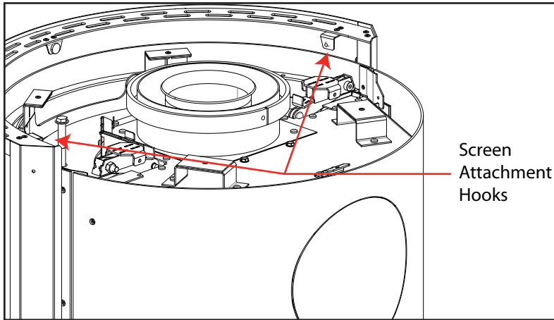
Figure 12: Safety Screen Attachment Hooks (Top Plate Removed for Visibility)
