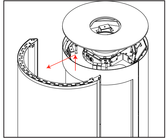
Figure 13: Safety Screen Removal
