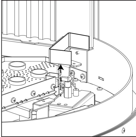
Figure 35: Pilot Fence Removal
