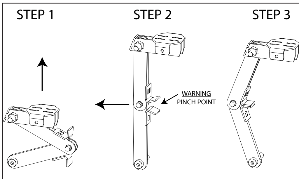
Figure 11: Top Plate Hinge Mechanism
