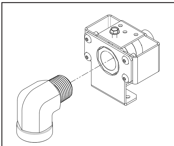
Figure 85: 1/2" Elbow Fitting Connection
