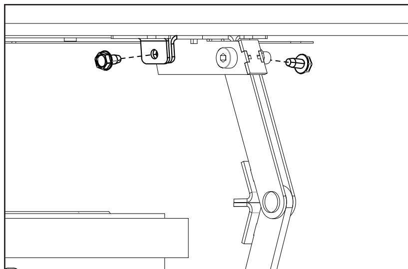
Figure 32: Top Plate Hinge Detachment
