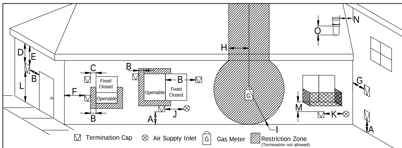
Figure 47: Vent Termination Restrictions, refer to Table 5.
