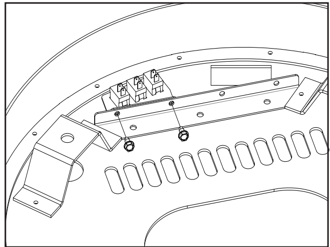
Figure 89: Rocker Switch Mount Attachment to Wood Pedestal
