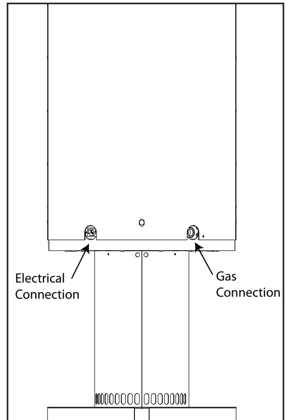
Figure 60: Electrical and Gas Connections
