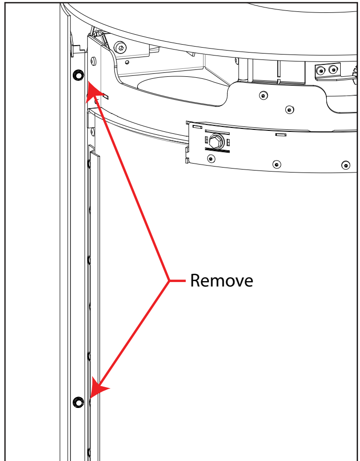
Figure 21: Rear Chassis Detachment
