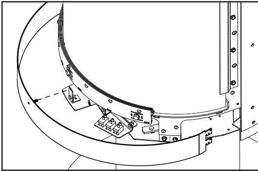
Figure 17: Front Skirt Attachment
