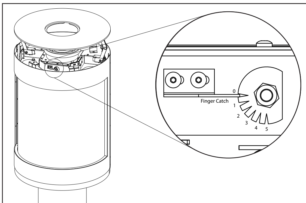
Figure 48: Exhaust Restrictor
