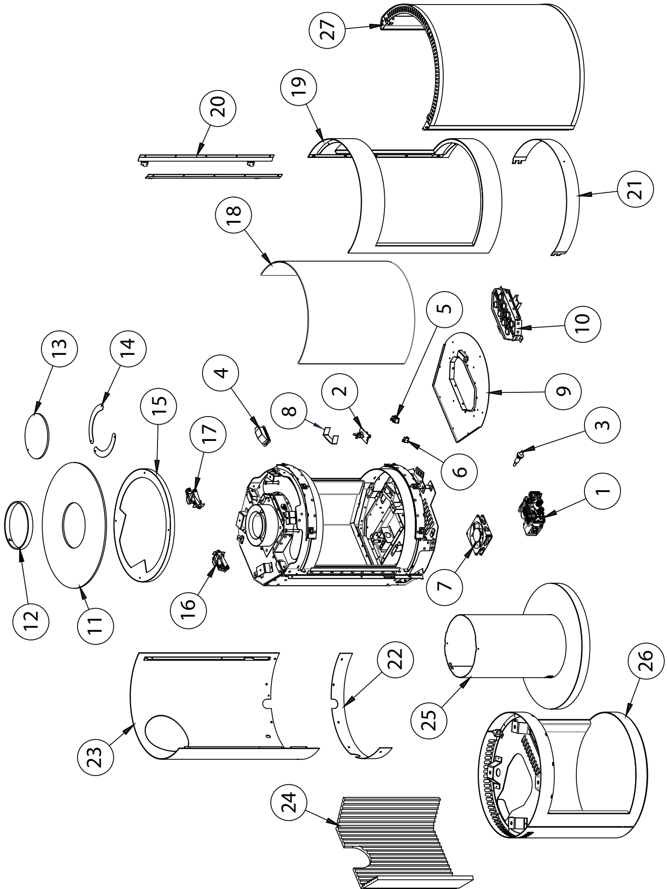
Figure 102: Parts List Diagram
