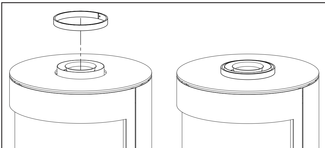
Figure 61: Top Plate Collar Placement
