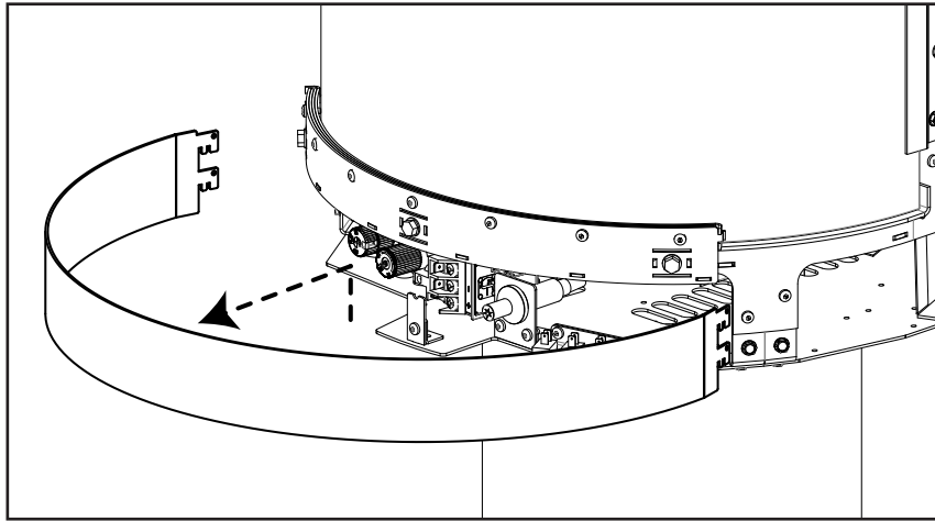
Figure 29: Front Skirt Removal
