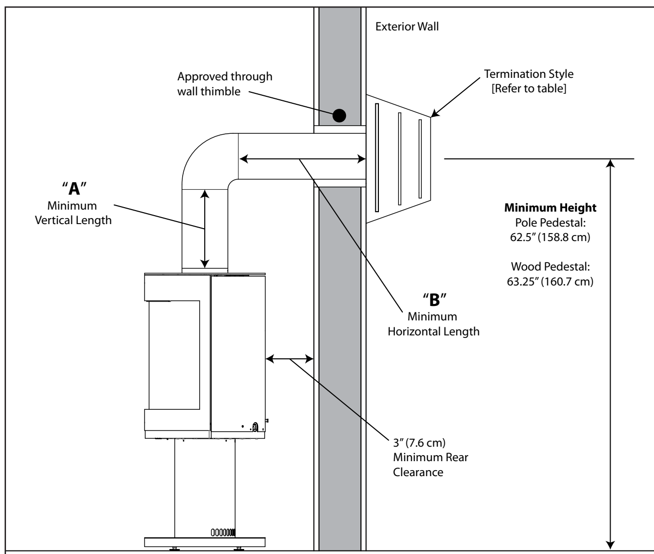
Figure 49: Minimum Vent Configuration - Top Vent
