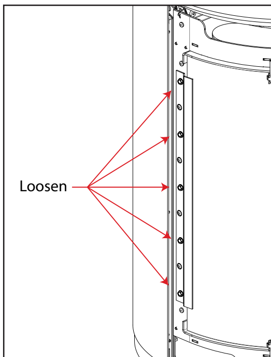
Figure 19: Glass Side Retainer
