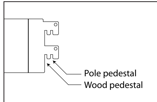
Figure 18: Front Skirt Attachment
