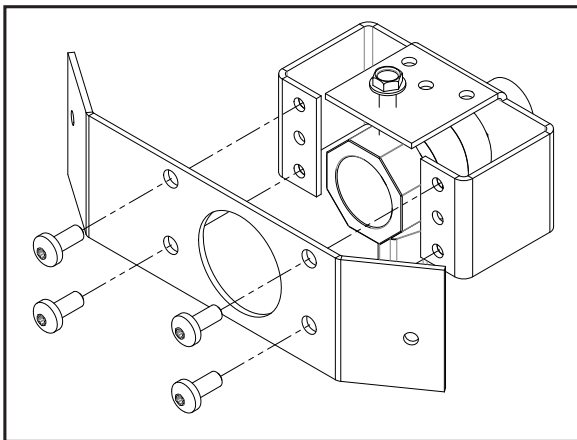
Figure 83: Gas Plate Removal
