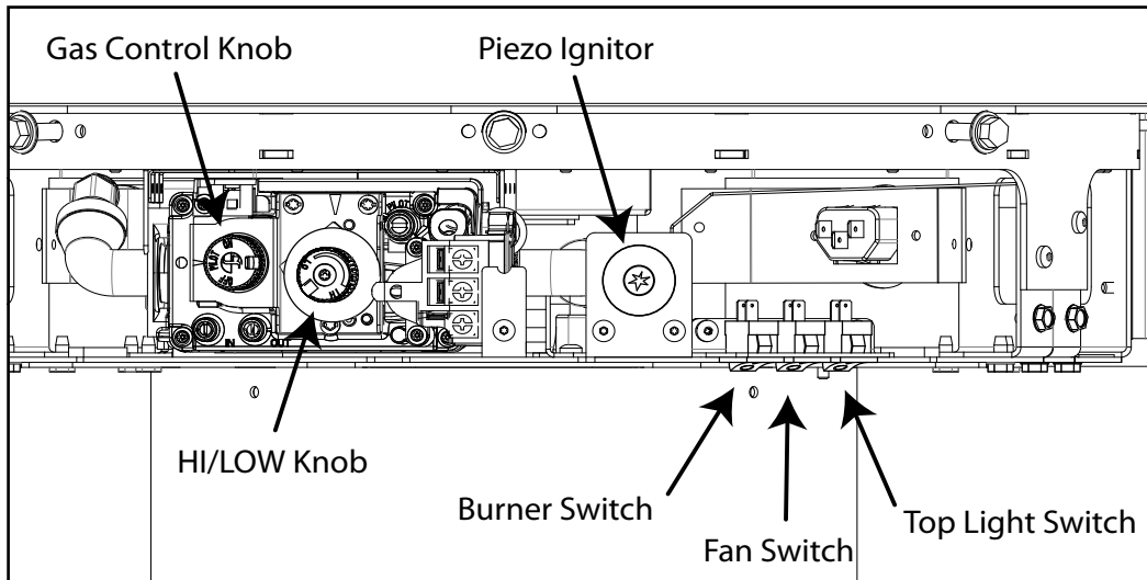
Figure 7: System Controls
