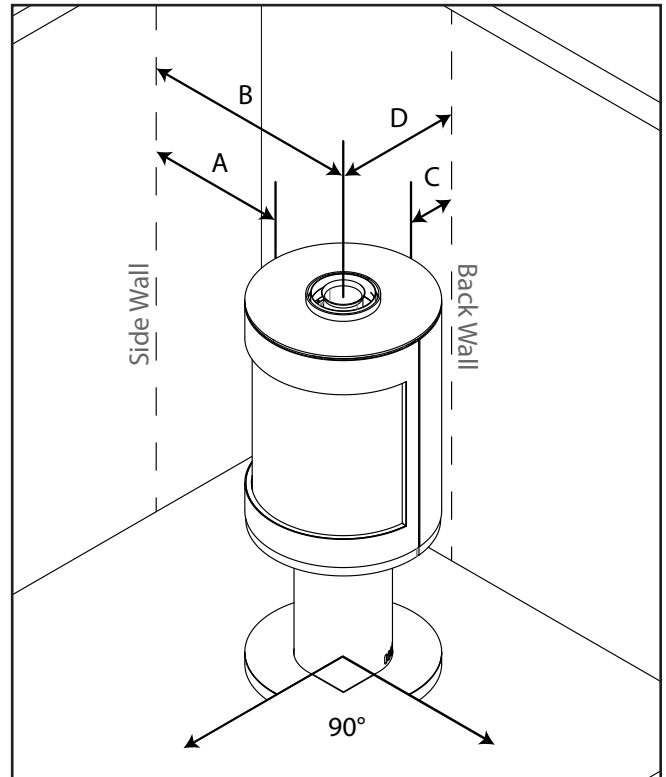
Figure 43: Clearance to Combustibles
