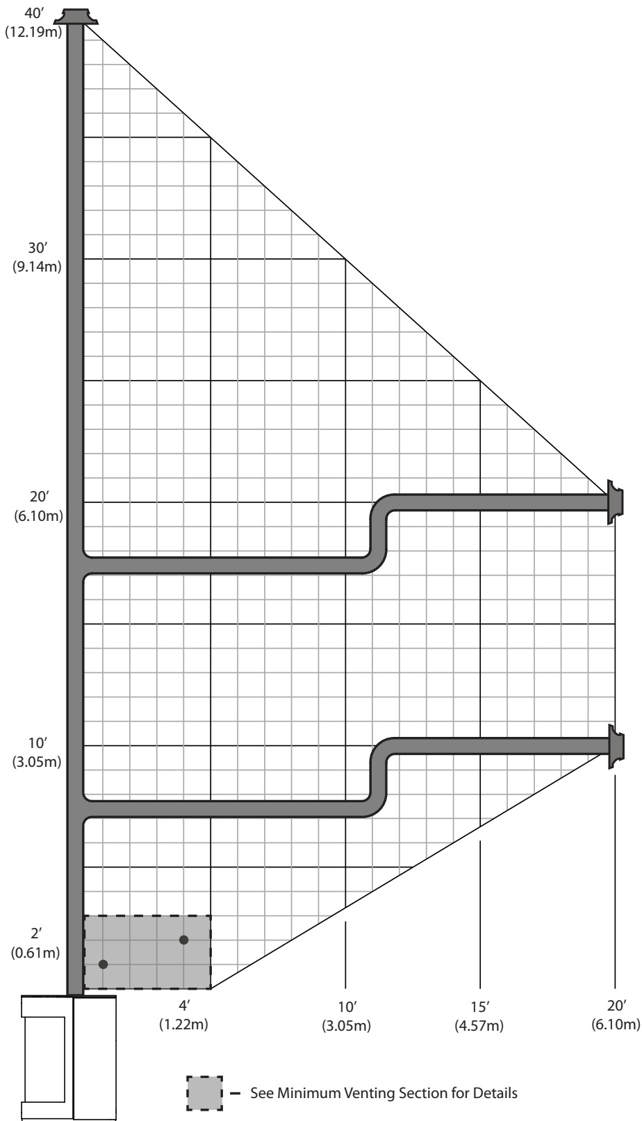
Figure 50: Top Vent Configuration Diagram - NG
