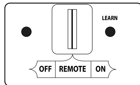
Fig. 25-2 Remote receiver detail (REMOTE)
