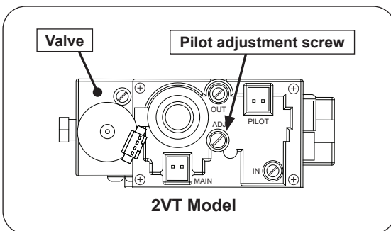
Fig. 33-4 Pilot Adjustment
