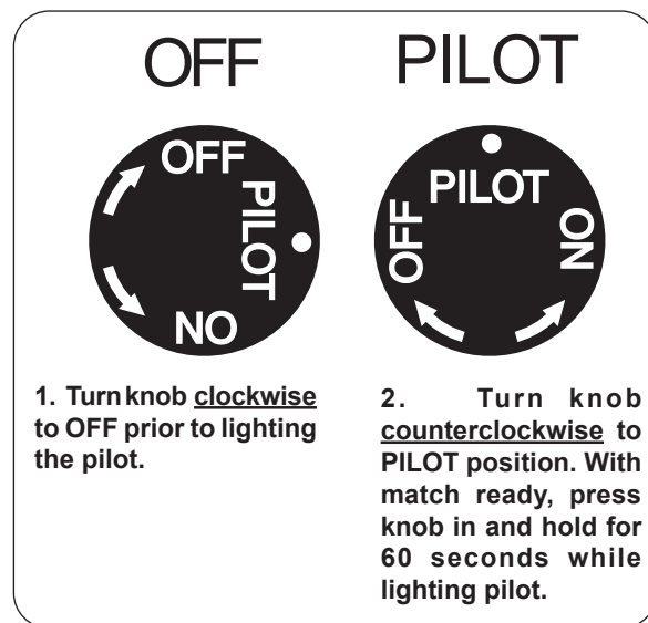
Fig. 25-1 Control knob detail (OFF, PILOT)
