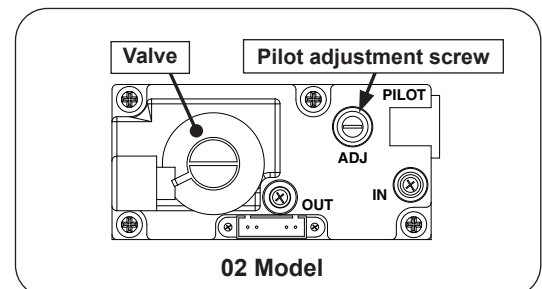
Fig. 39-3 Pilot Adjustment
