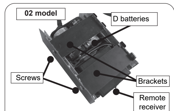
Fig. 20-2 Remote receiver batteries
