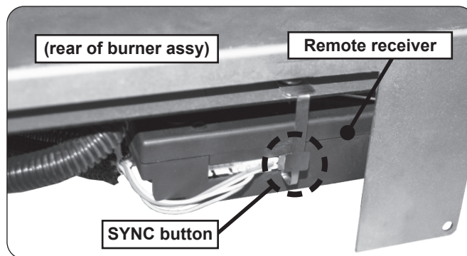
Fig. 42-2 Sync detail
