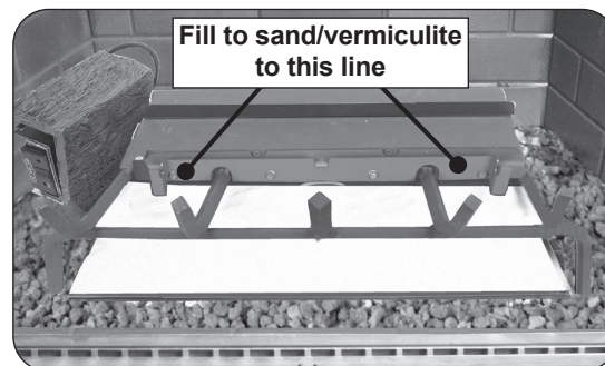
Fig. 16-3 Place sand/vermiculite
