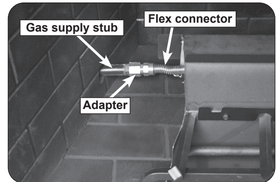
Fig. 15-1 Connect gas supply
