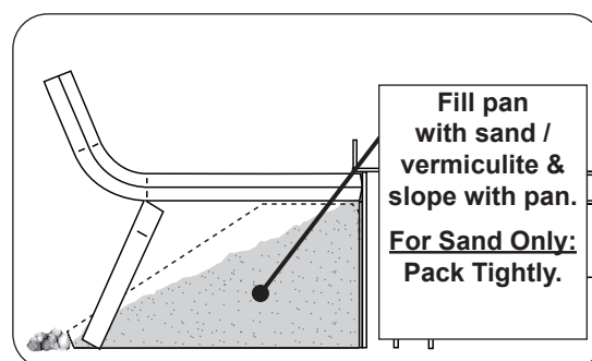
Fig. 16-4 Sand/vermiculite detail
